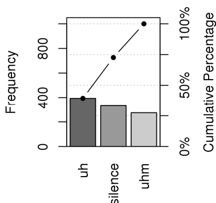
Figure 23. Pareto-chart with the frequencies of disfluencies
