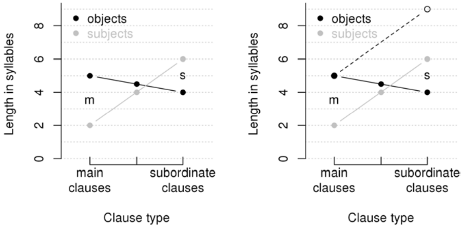
Figure 58. Interaction plot for \text{LENGTH} \sim \text{GRMRELATION} * \text{CLAUSETYPE } 2
