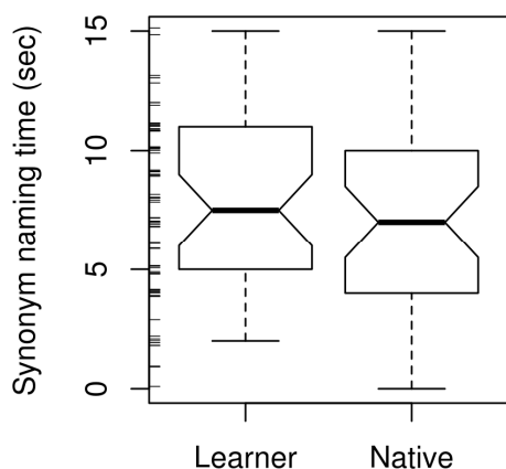
Figure 47. Boxplot for SYNTIMES~SPEAKER
