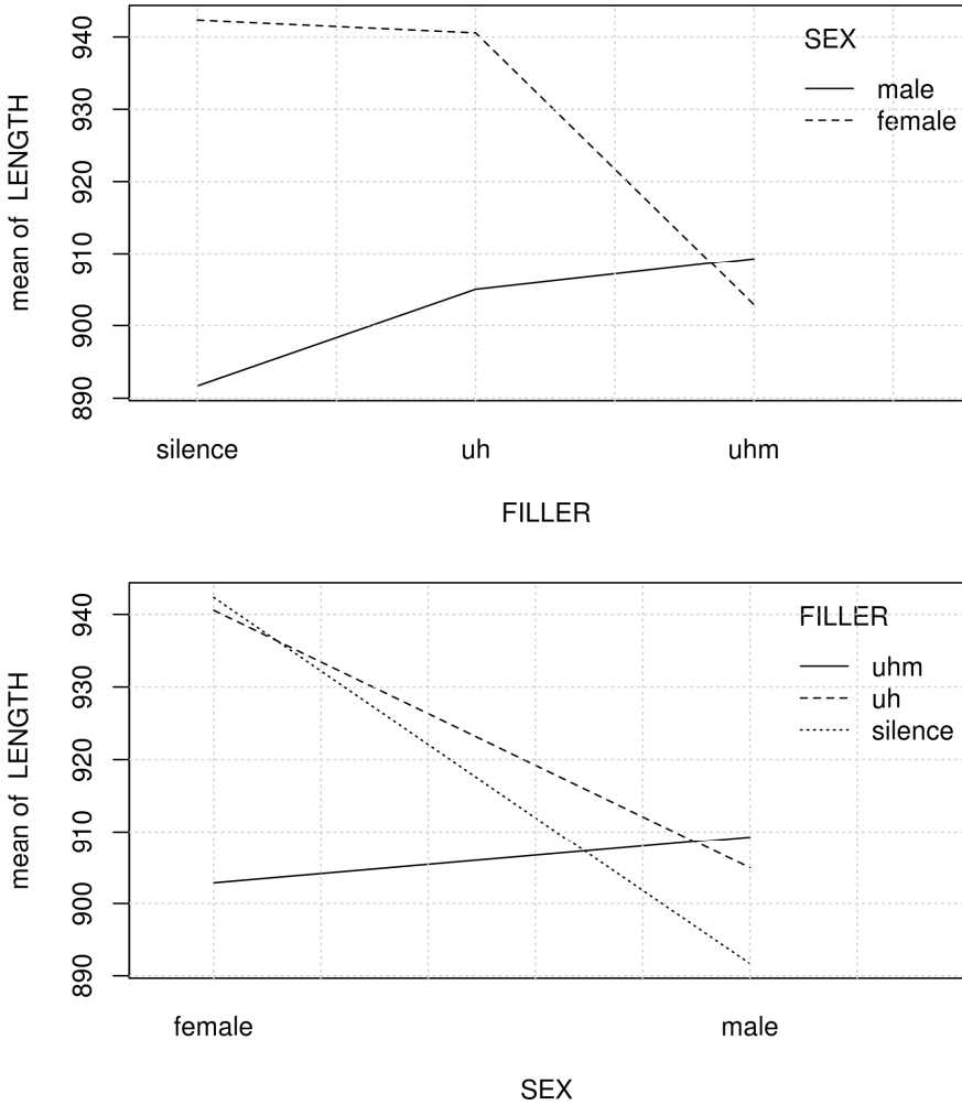
Figure 34. Interaction plot for LENGTH \sim FILLER : SEX
